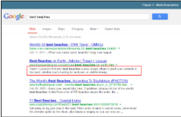
Figure 1 - Meta Description
